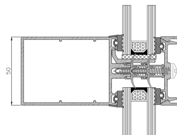
Transom section
