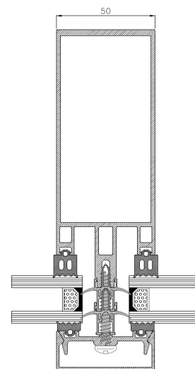
Upright section
